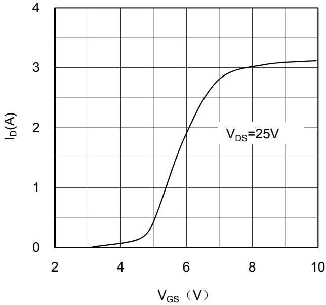
Figure 1. Transfer characteristics
